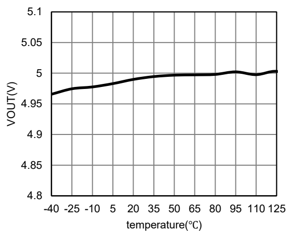
VOUT@200mA VS Temperature
