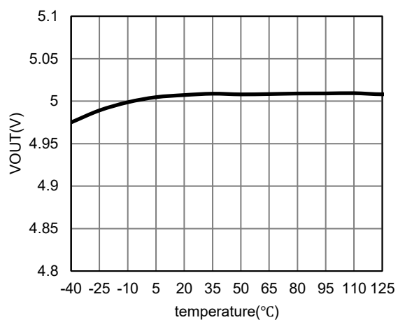
VOUT@1mA VS Temperature
