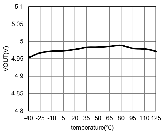
VOUT@500mA VS Temperature
