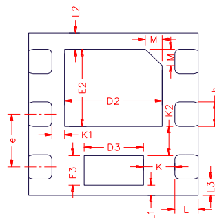
BOMTTOM VIEW
