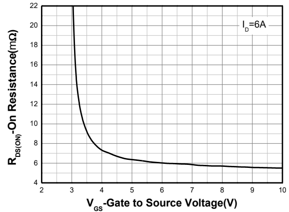
On-Resistance vs. Gate-to-Source Voltage d
